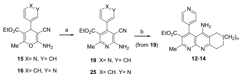
Scheme 5. Reagents and conditions: (a) \text{AcOH} , \text{AcONH}_4 ( 15–19 : 57%), ( 16–25 : 15%); (b) 1,2-dichloroethane, \text{AlCl}_3 , cyclopentanone ( 12 , n = 0 , 61%); cyclohexanone ( 13 , n = 1 , 49%), cycloheptanone ( 14 , n = 2 , 92%).
