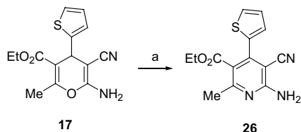
Scheme 6. Reagents and conditions: (a) AcOH, AcONH 4 (5%).
