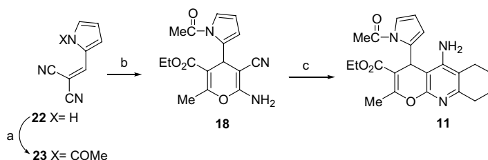
Scheme 4. Reagents and conditions: (a) \text{Ac}_2\text{O} , py (98%); (b) ethyl acetoacetate, piperidine (99%); (c) 1,2-dichloroethane, \text{AlCl}_3 , cyclohexanone (43%).
