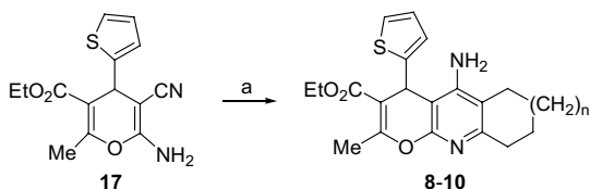
Scheme 2. Reagents and conditions: (a) 1,2-dichloroethane, \text{AlCl}_3 , cyclopentanone ( 8 , n = 0 , 29%); cyclohexanone ( 9 , n = 1 , 83%), cycloheptanone ( 10 , n = 2 , 61%).
