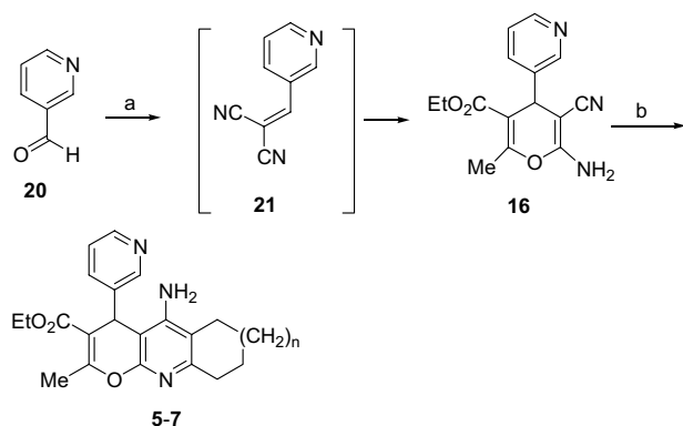
Scheme 3. Reagents and conditions: (a) malononitrile, then ethyl acetoacetate, piperidine (84%); (b) 1,2-dichloroethane, \text{AlCl}_3 , cyclopentanone ( 5 , n = 0 , 73%); cyclohexanone ( 6 , n = 1 , 88%), cycloheptanone ( 7 , n = 2 , 77%).
